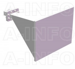
LB-187-20-C-3.5FSP0 Standard Gain Horn Antenna 3.95-5.85GHz 20dB Gain 3.5mm Female
